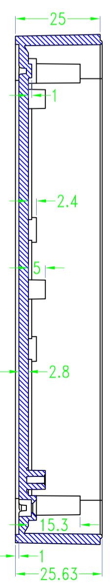
SEC B-B
